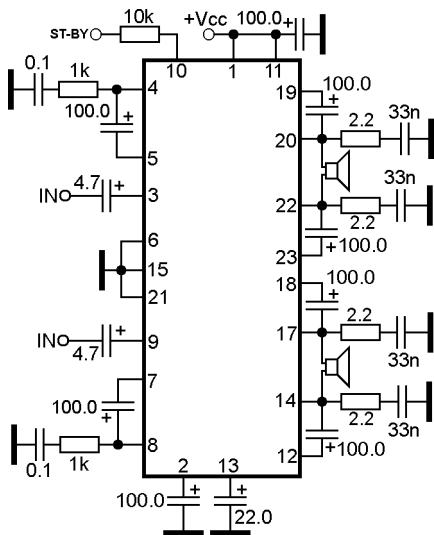
Dual power audio amplifier with stand-by
