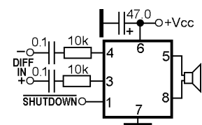
BTL class-D power audio amplifier with shutdown
