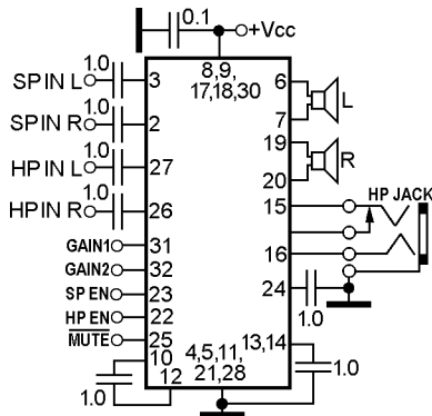
Dual BTL (speaker) and SE (headphone) power audio amplifier with separate enable, gain select and mute
