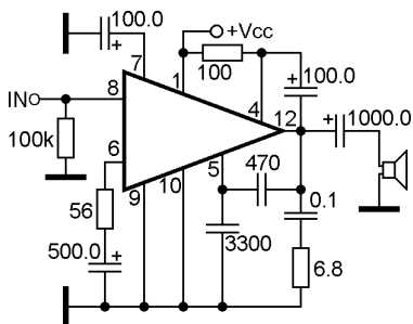
SE mode (standard) sample application circuit
