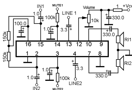
Dual power audio amplifier for headphone with internal LPF for CD-ROM
