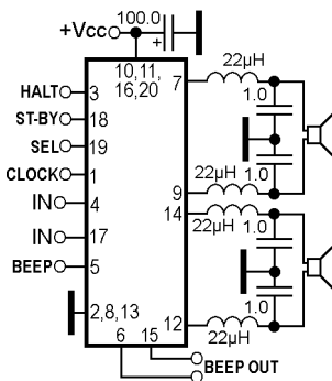
Dual class-D power audio amplifier for headphone with logic control, external clock and internal LDO voltage regulator
