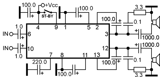
Dual power audio amplifier with stand-by
