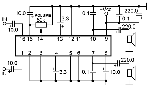
Stereo SE mode sample application circuit
