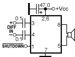
BTL class-D power audio amplifier with differential input, fixed gain and shutdown
