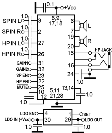
Dual BTL (speaker) and SE (headphone) power audio amplifier with separate enable, gain select and mute
