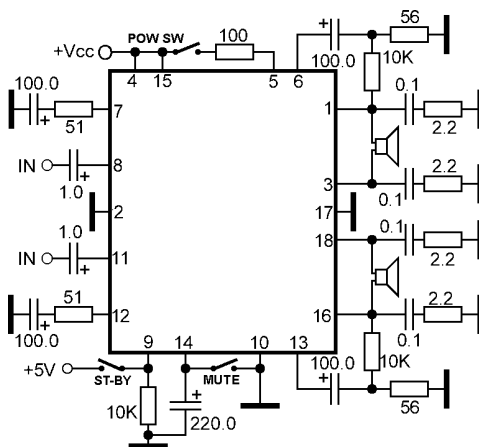
Dual BTL power audio amplifier with mute and stand-by
