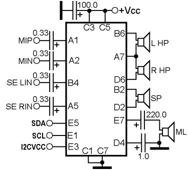
BTL (speaker), dual SE (headphone), BTL (earpiece) power audio amplifier with I2C-bus control
