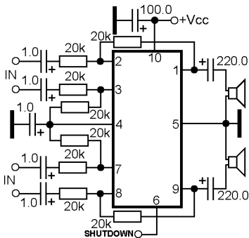
Dual power audio amplifier for headphone with differential inputs and shutdown
