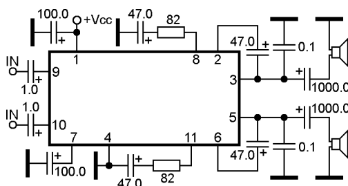
Standard (dual SE) sample application circuit
