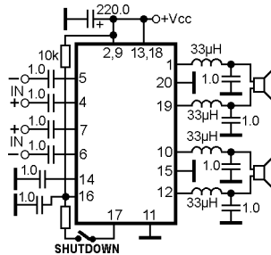
Dual class-D power audio amplifier with shutdown
