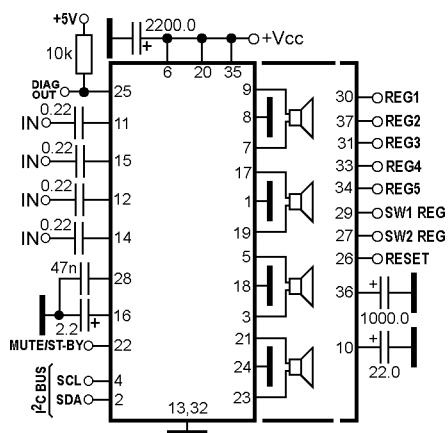
Quad BTL power audio amplifier with mute/stand-by, I2c-bus control, multiple voltage regulators and diagnostic facility
