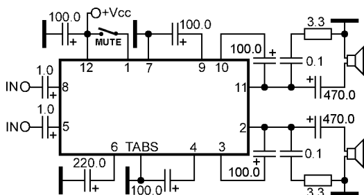
Dual power audio amplifier with mute
