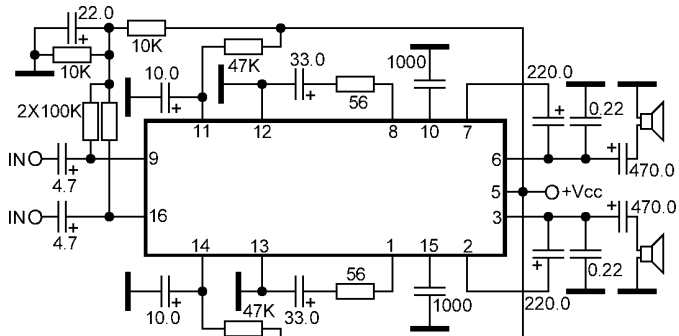
Dual power audio amplifier for headphone
