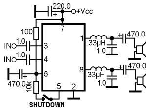
Dual class-D power audio amplifier with shutdown
