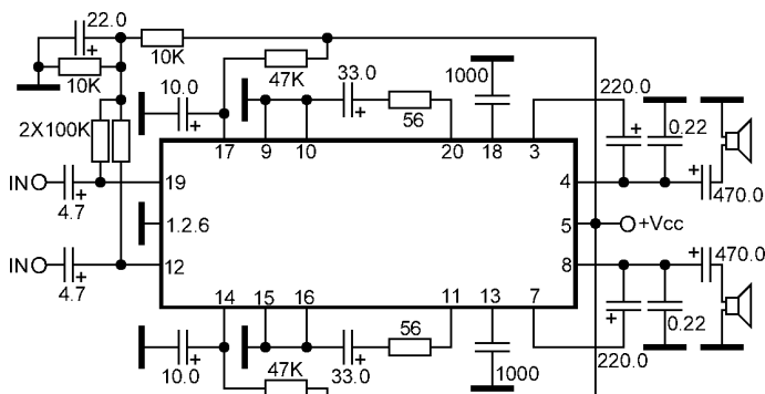
Dual power audio amplifier for headphone
