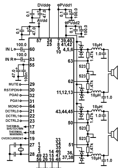
Dual BTL mode sample application circuit
