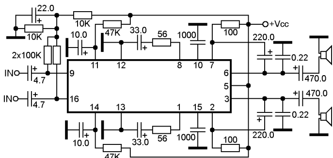
Dual power audio amplifier for headphone
