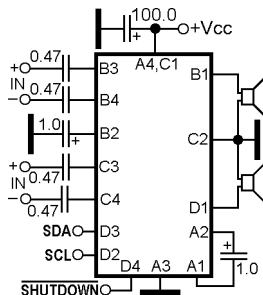
Dual power audio amplifier for headphone with differential inputs, shutdown and I2C control
