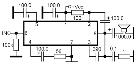
Power audio amplifier with microphone input for hearing instrument
