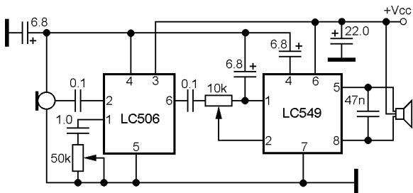
Power audio amplifier for hearing instrument
