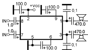
Dual power operational/audio amplifier
