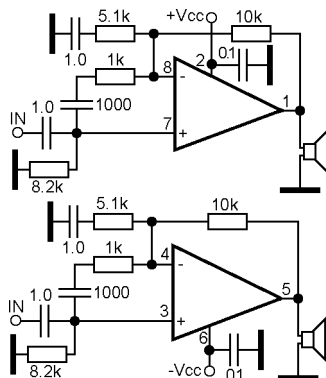
Standard (dual SE) sample circuit diagram
