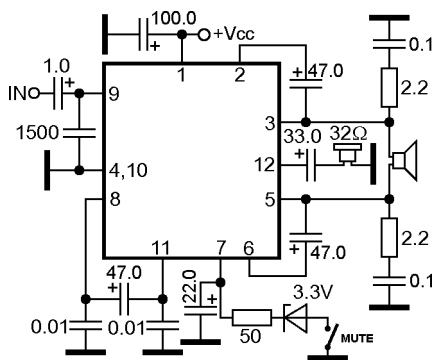
BTL mode sample application circuit
