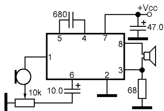
Power audio amplifier with microphone input for hearing instrument
