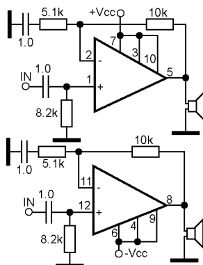
Dual power operational/audio amplifier
