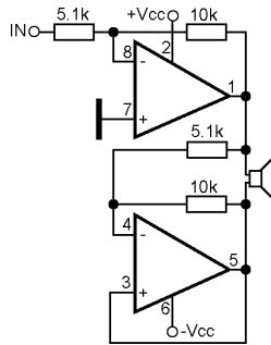
BTL mode sample circuit diagram
