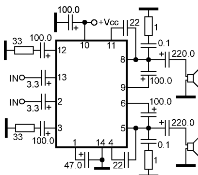
Dual power audio amplifier
