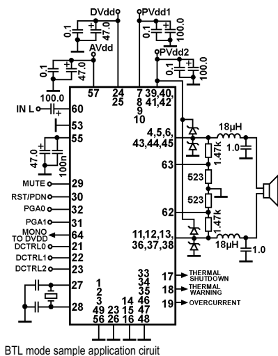
BTL mode sample application circuit
