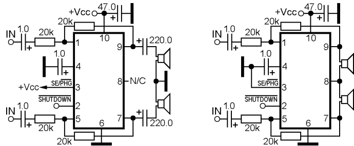
Dual power audio amplifier for headphone with shutdown
