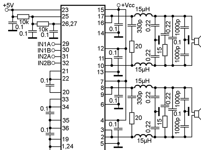
Dual BTL class-T power audio amplifier output stage with differential inputs
