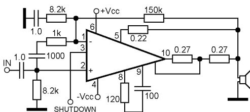
Power operational/audio amplifier
