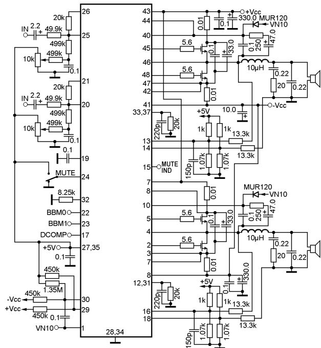
Power audio amplifier
