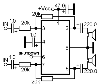
Dual power audio amplifier for headphone with shutdown
