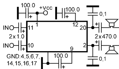
Dual power audio amplifier with stand-by
