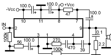
Power audio amplifier
