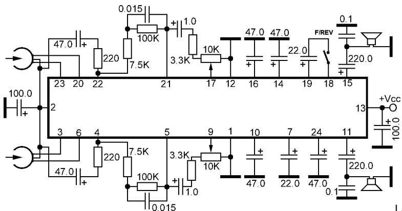
Dual playback preamplifier for autoreverse, power audio amplifier for headphone
