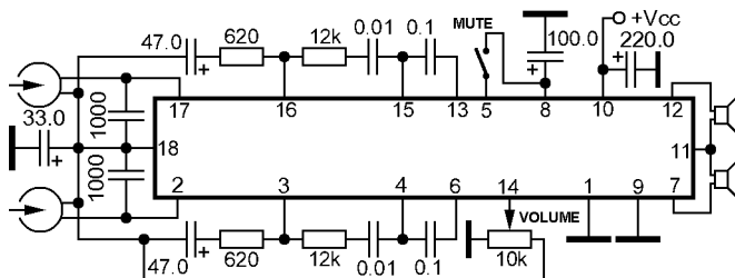
Dual playback preamplifier, volume control, power audio amplifier for headphone
