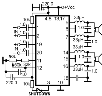
Dual BTL class-D power audio amplifier with differential inputs, DC volume control and shutdown
