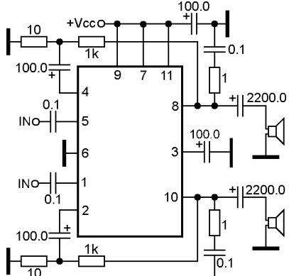
Dual SE mode without bootstrap sample application circuit
