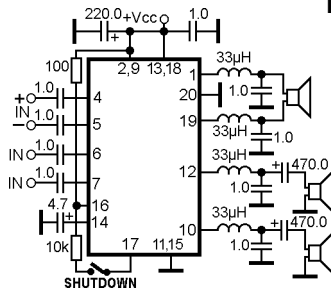
Triple (dual SE and BTL) class-D power audio amplifier with shutdown
