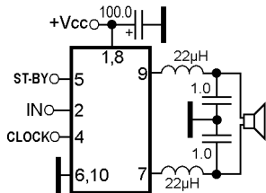
BTL class-D power audio amplifier output stage for headphone with external clock
